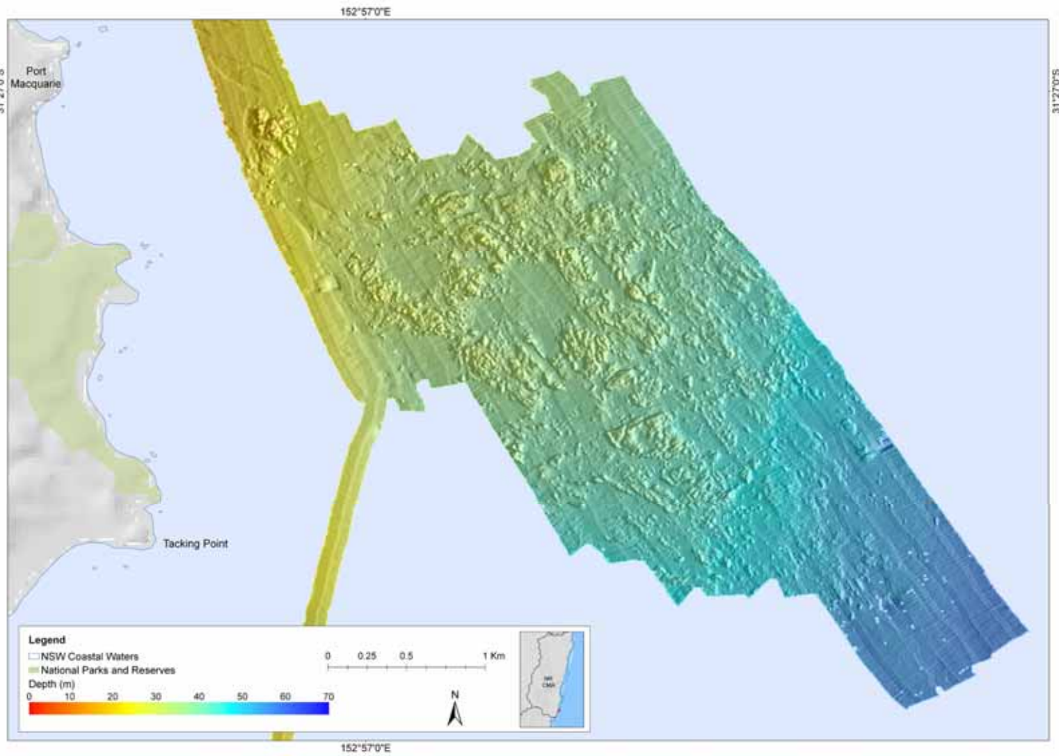
Figure 59. Hill-shaded bathymetric model of the seabed offshore of Port Macquarie.
