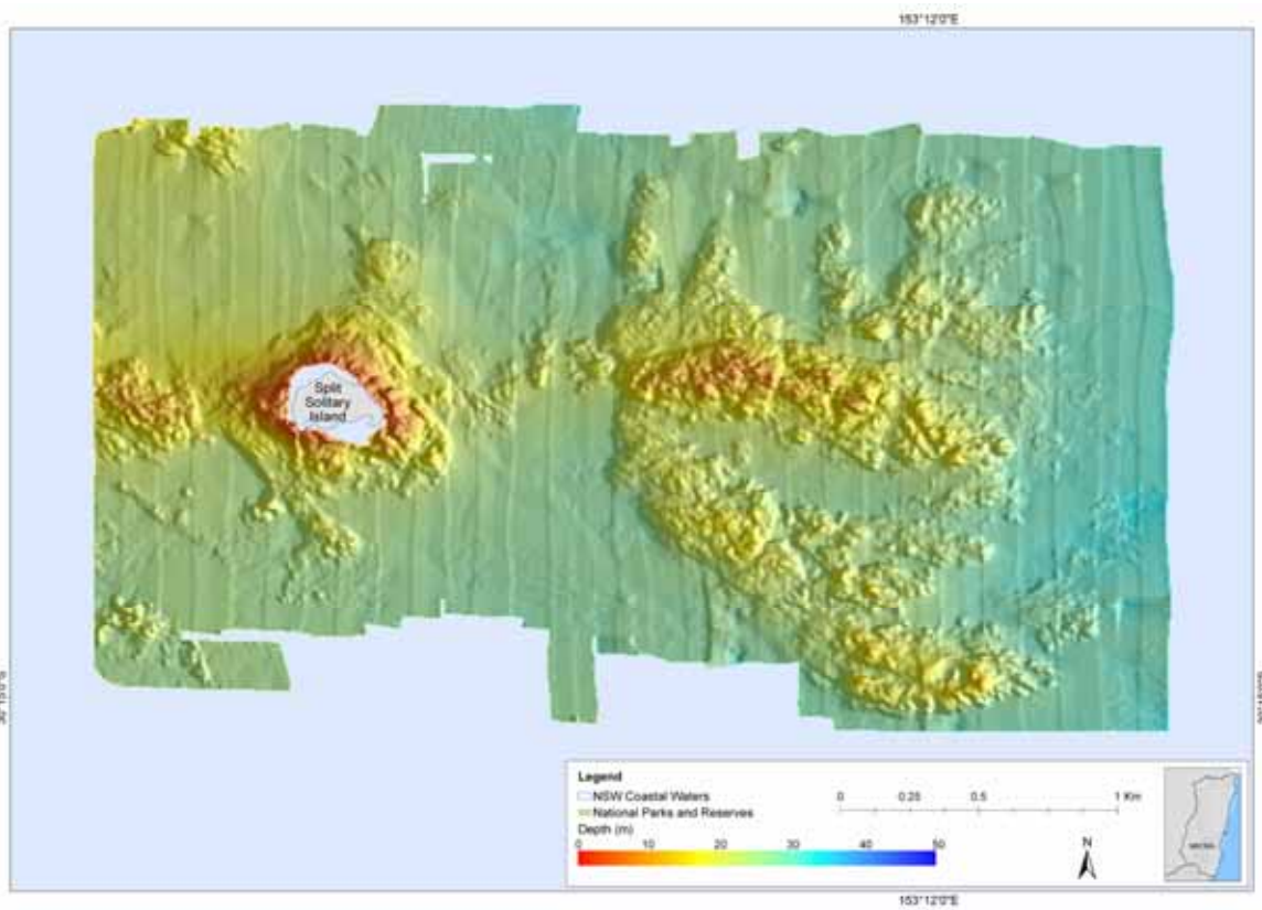
Figure 34. Hill-shaded bathymetric model of the seabed adjacent to and east of Split Solitary Island.
