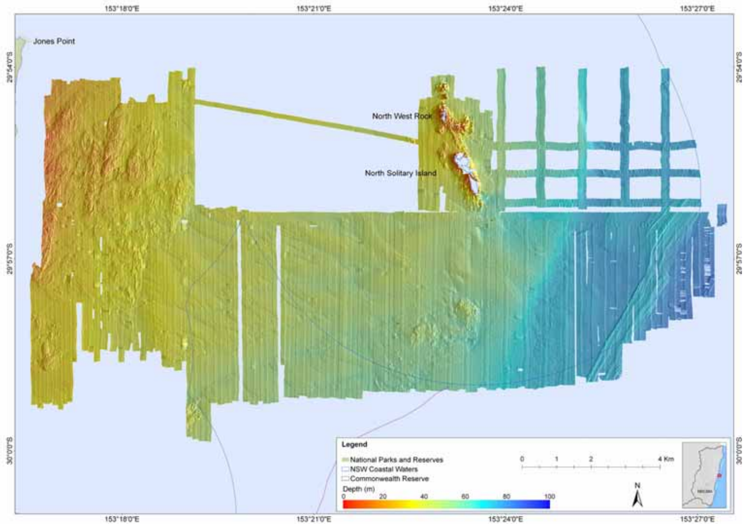
Figure 20. Hill-shaded bathymetric model of the seabed offshore of Jones Point and North Solitary Island.
