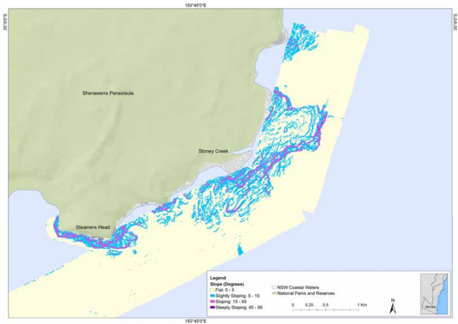
Figure 126. Slope model of the seabed adjacent to the Bherwerre Peninsula between Steamers Head and the southern section of Governors Head.
