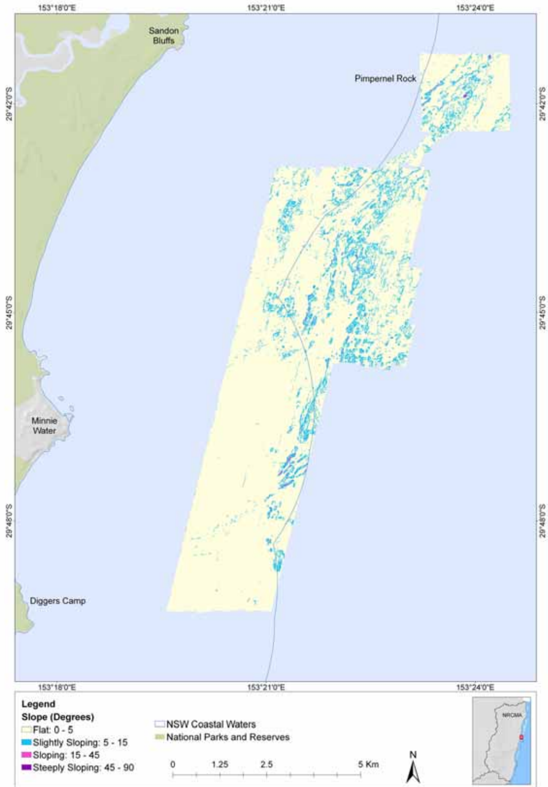
Figure 18. Slope model of the seabed offshore of the Minnie Waters region and within the Solitary Islands Marine Reserve (Commonwealth waters).
