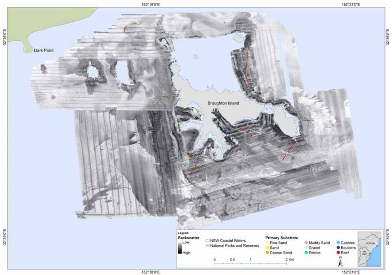
Figure 103. Acoustic backscatter of the seabed surrounding Broughton Island.
