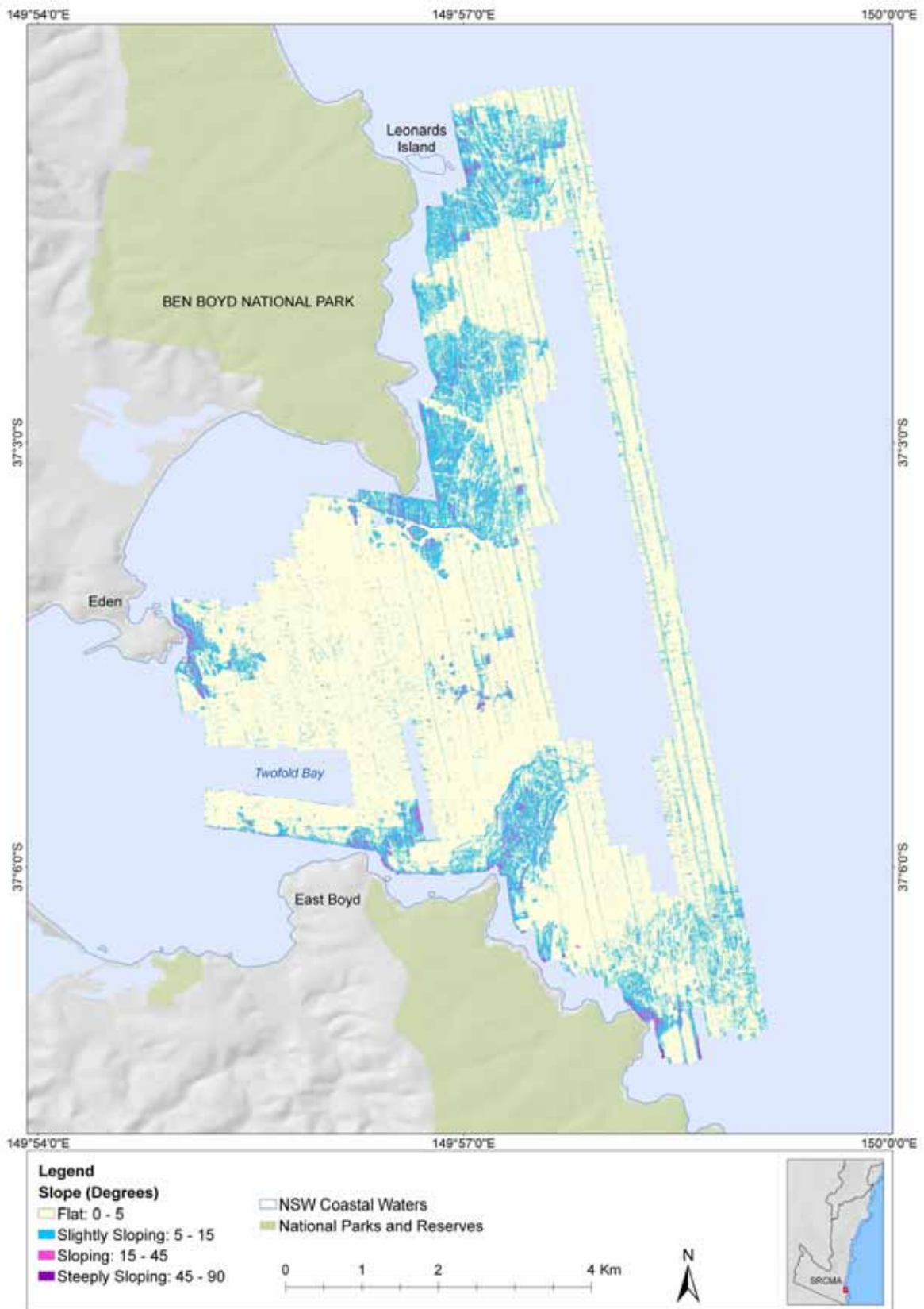
Figure 150. Slope model of the seabed within the Twofold Bay region.
