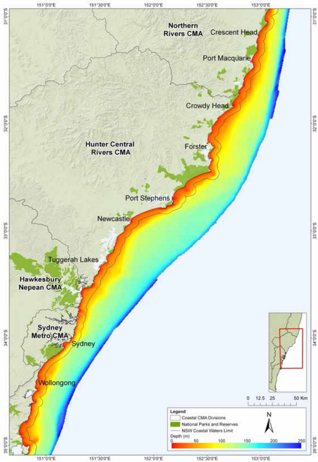
Figure 8. Interpolated broadscale bathymetry of the central and Sydney continental shelf regions of NSW (HCRCA, HNCMA and SMCMA regions). CMA, catchment management authority.
