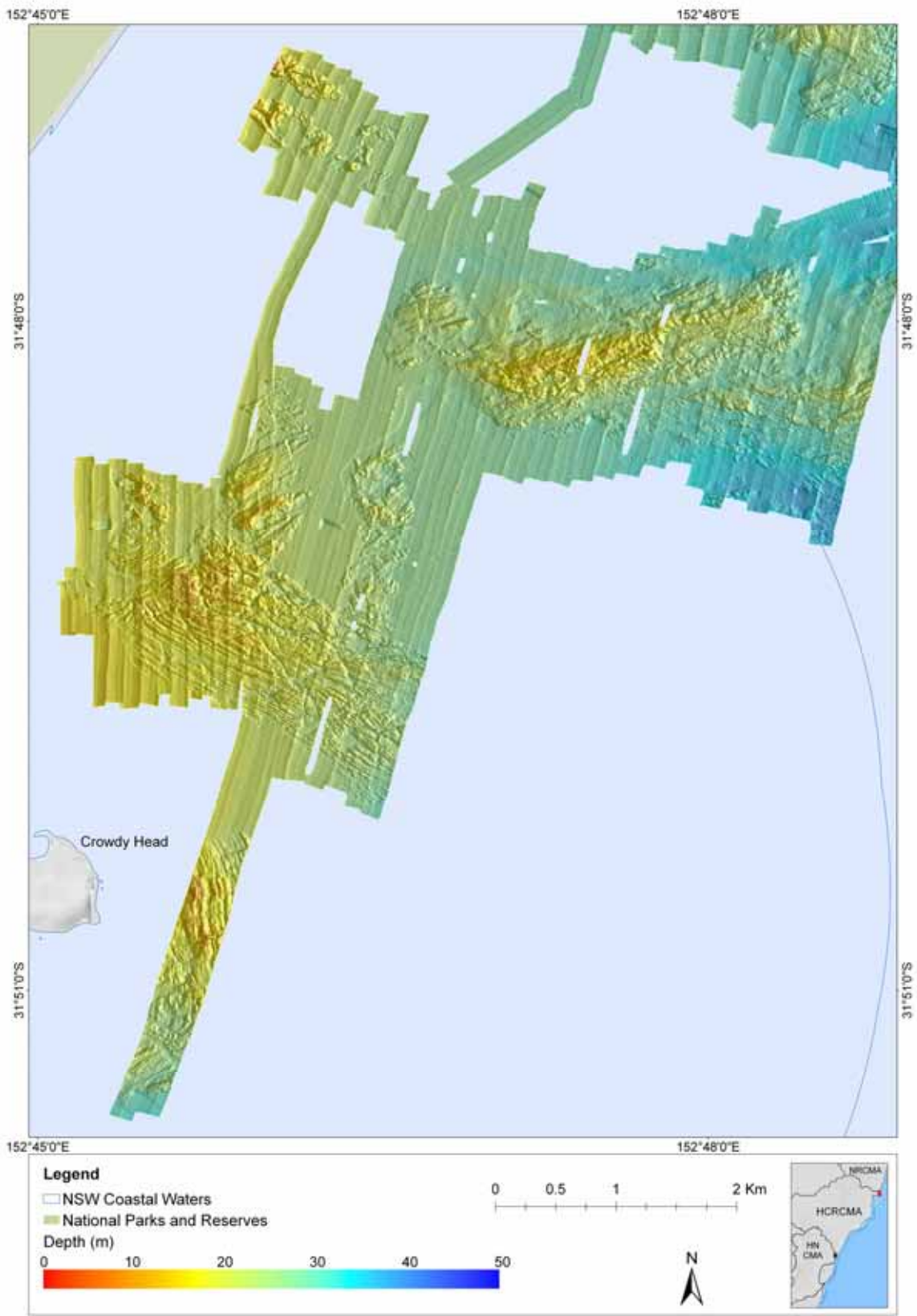
Figure 74. Hill-shaded bathymetric model of the seabed from the Giles Shoal and Curphy Shoal regions.
