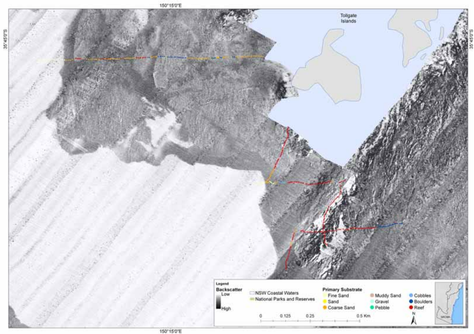
Figure 135. Acoustic backscatter of the seabed south of the Tollgate Islands region.
