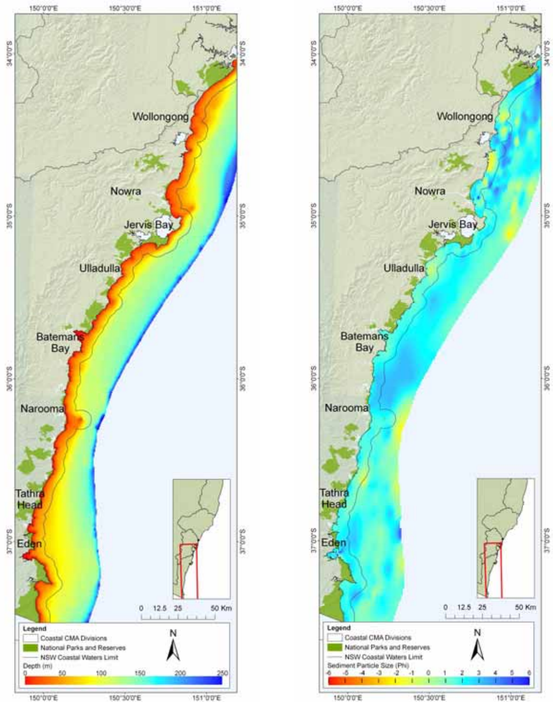
Figure 10. Interpolated broadscale bathymetry and surficial sediment distribution of the southern continental shelf region of NSW (Southern Rivers CMA region). CMA, catchment management authority.
