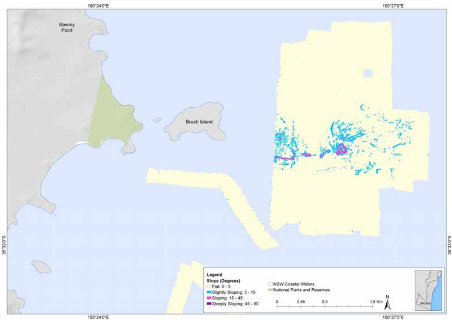
Figure 130. Slope model of the seabed adjacent to the Brush Island region.
