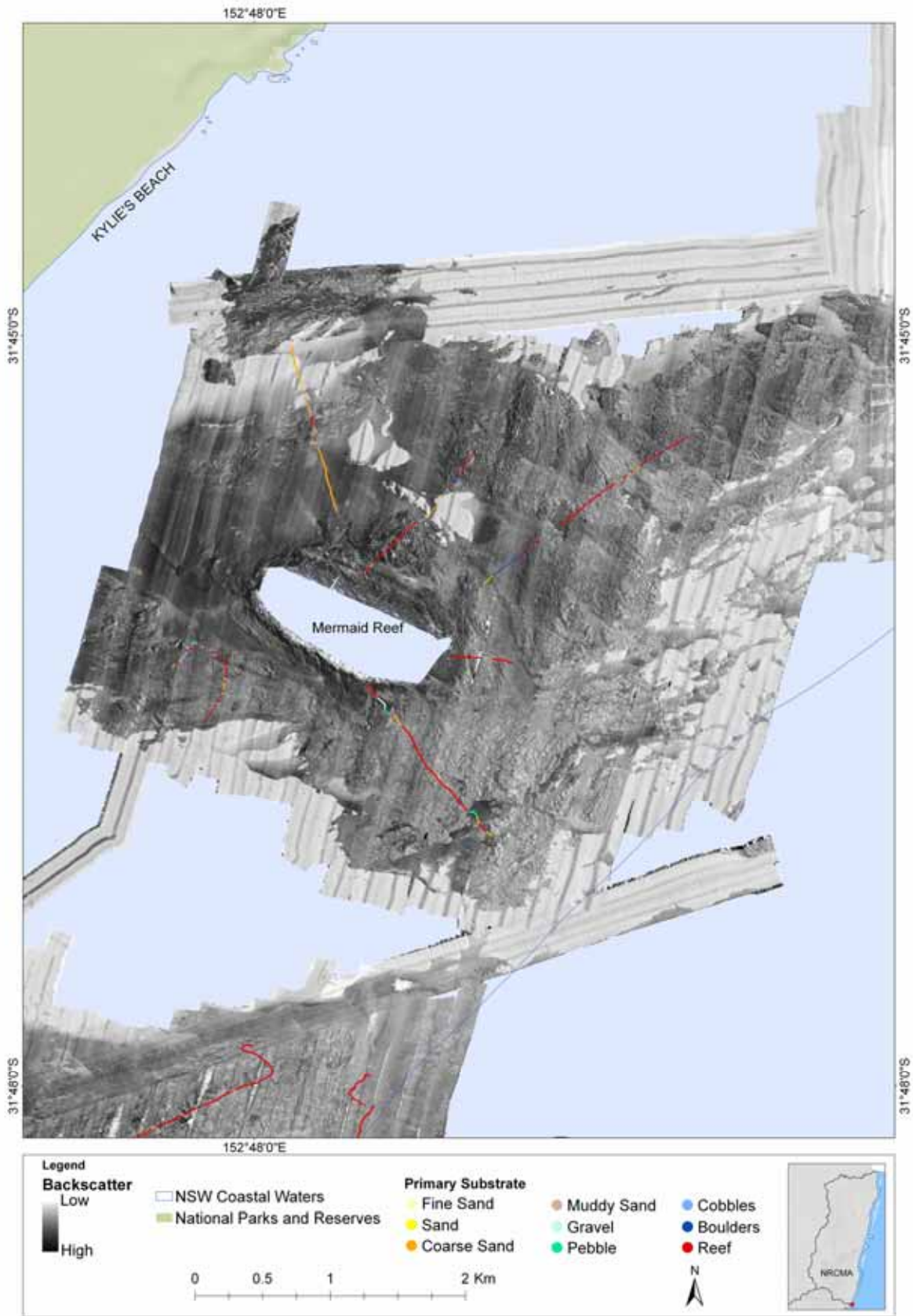
Figure 73. Acoustic backscatter of the seabed of the Mermaid Reef region offshore of Crowdy Head.
