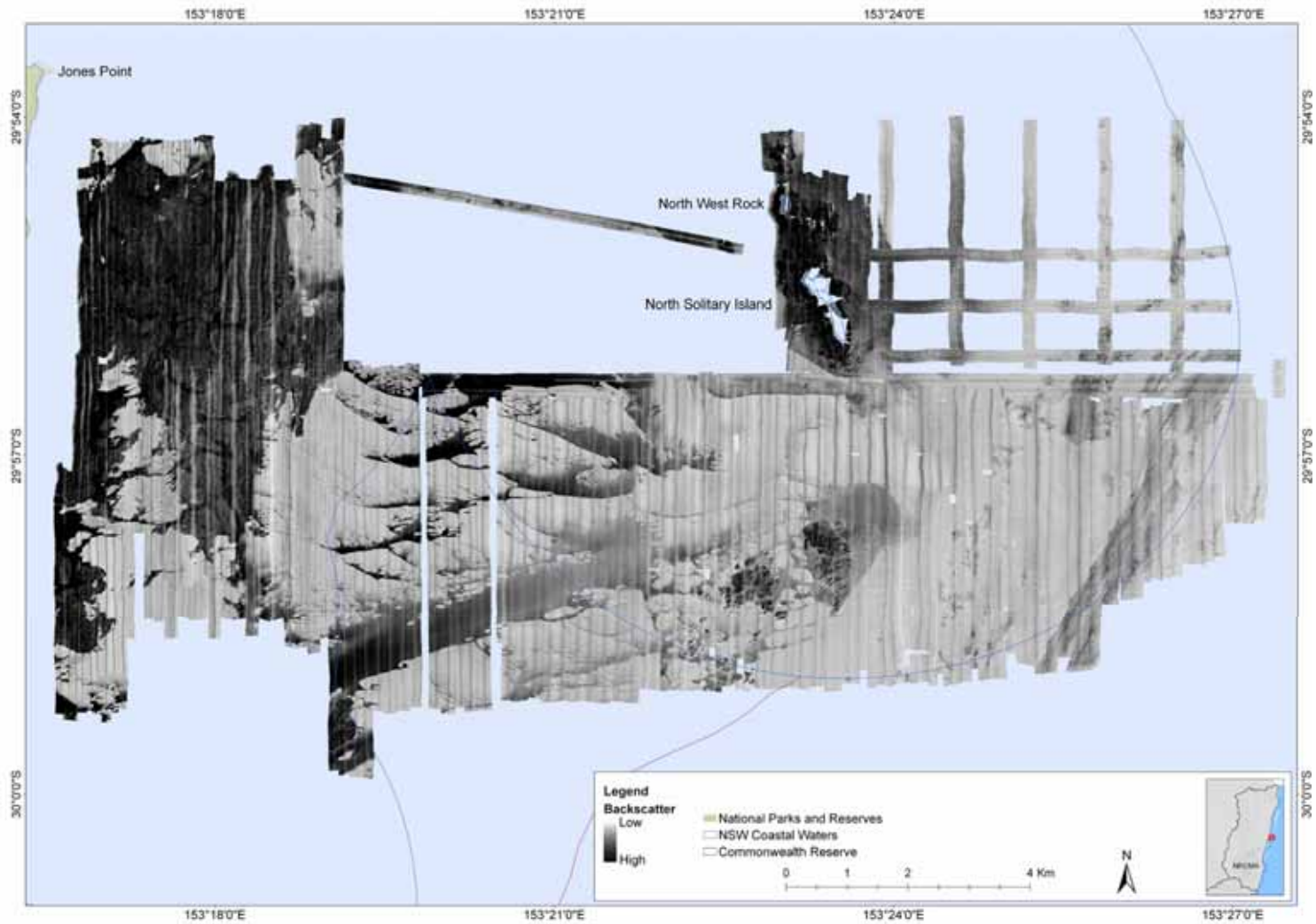
Figure 22. Acoustic backscatter of the seabed offshore of Jones Point and North Solitary Island.
