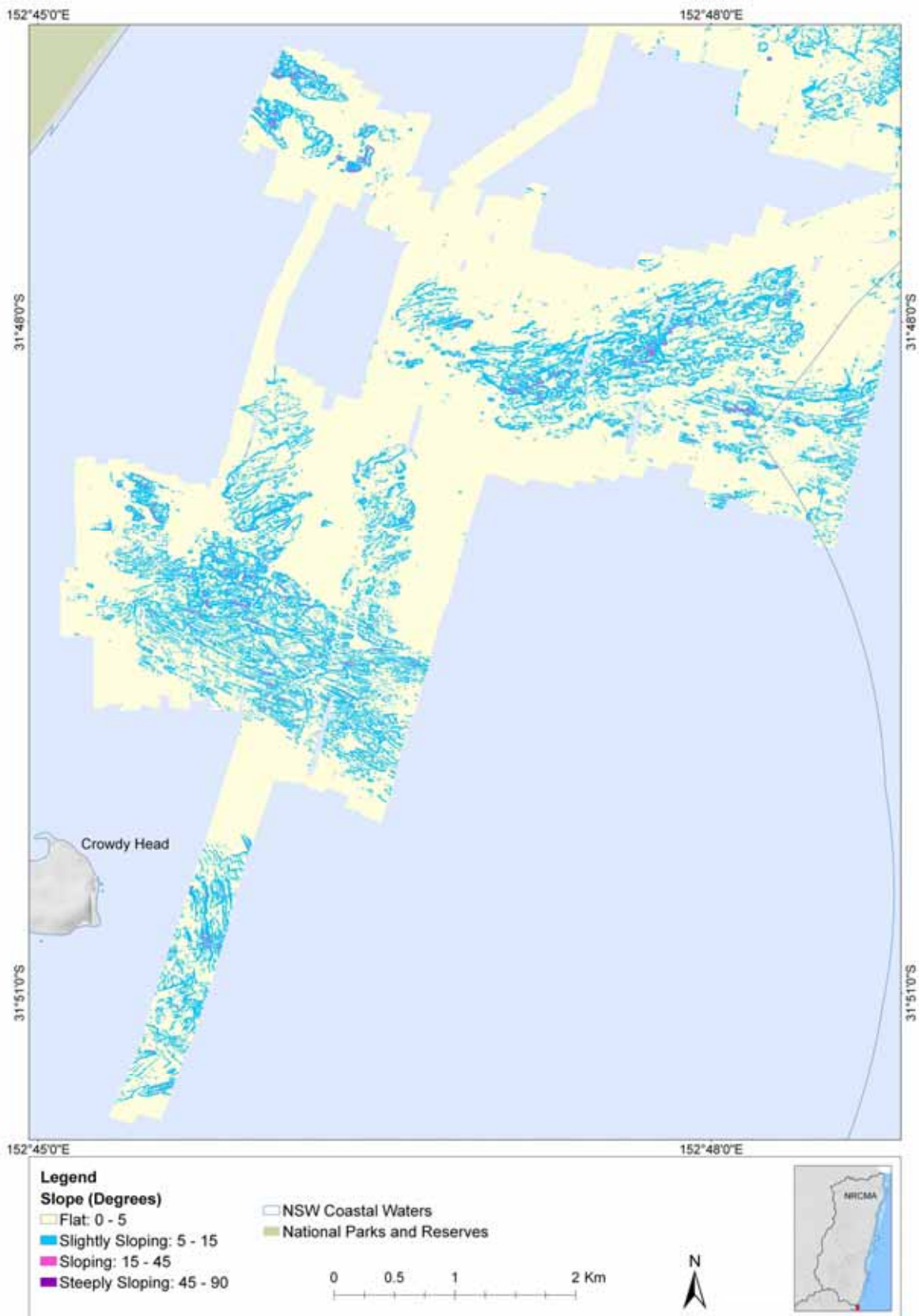
Figure 75. Slope model of the seabed of the Giles Shoal and Curphy Shoal regions offshore of Crowdy Head.
