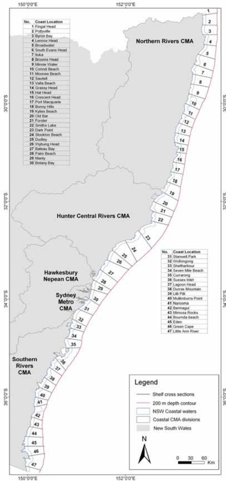
Figure 1. Position of transects used to estimate continental shelf distances and depths from the broadscale bathymetry.
