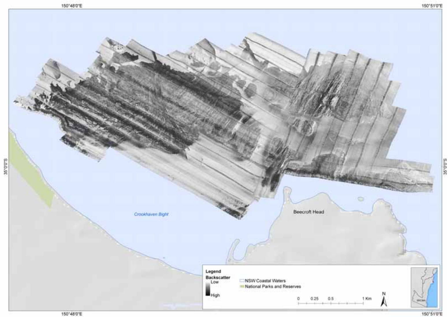
Figure 121. Acoustic backscatter of the seabed within Crookhaven Bight.
