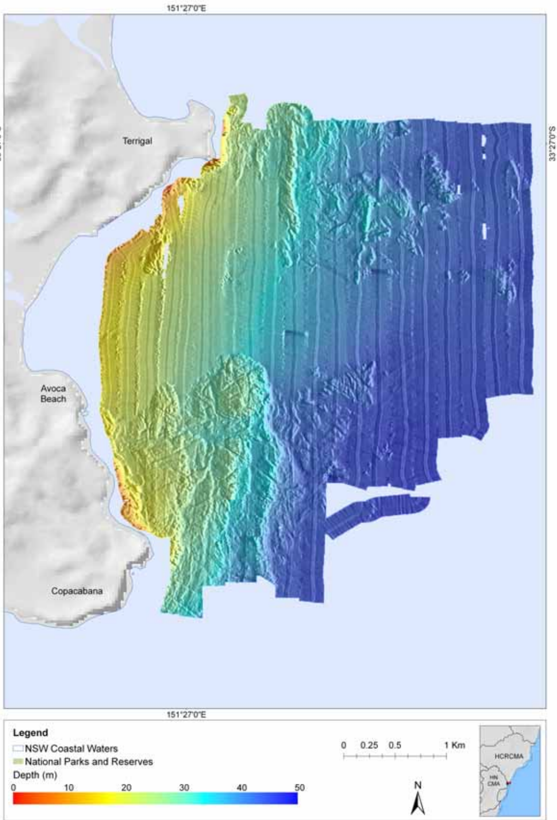
Figure 113. Hill-shaded bathymetric model of the seabed offshore of Terrigal.
