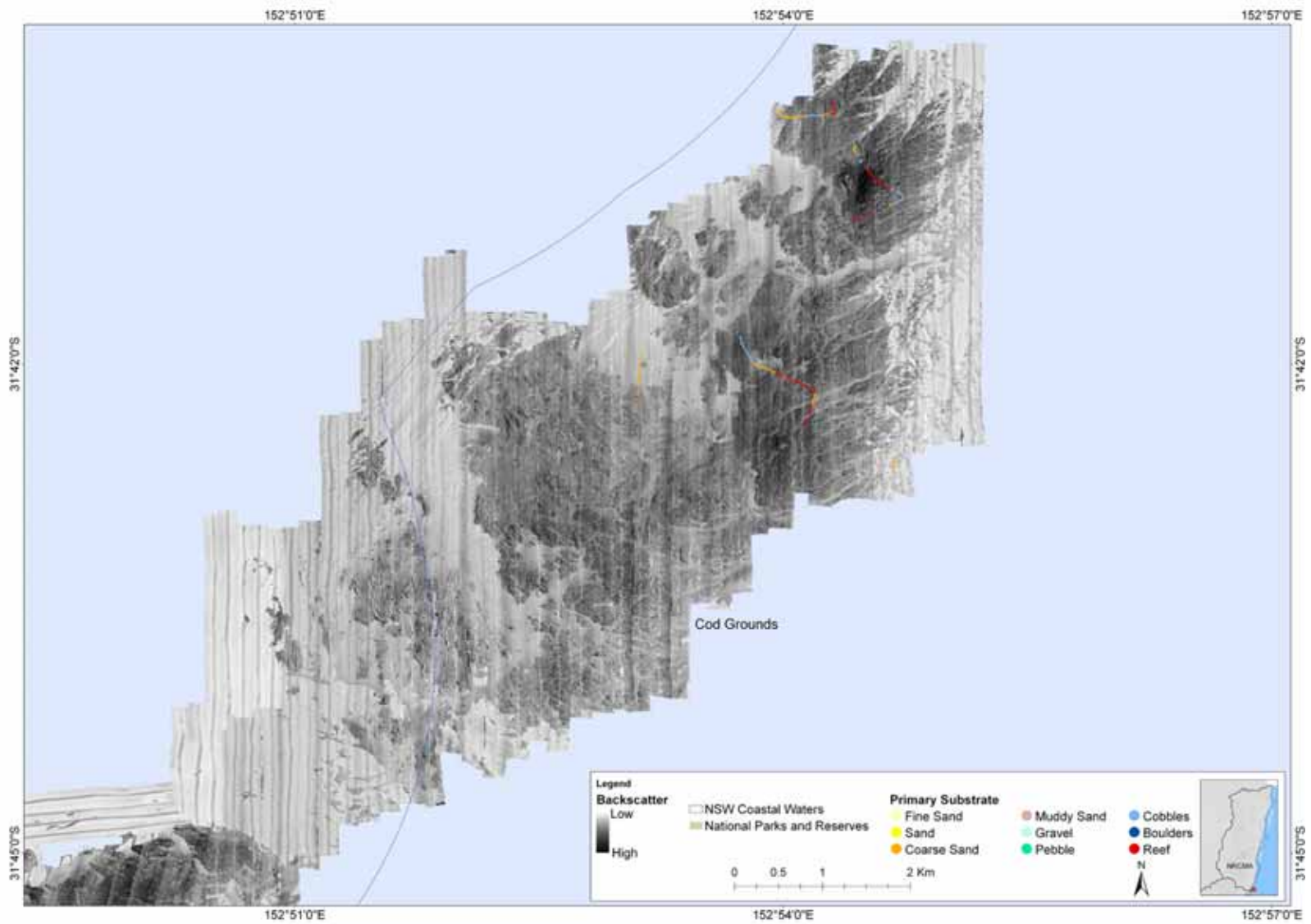
Figure 70. Acoustic backscatter of the seabed offshore of the region between Perpendicular Point and Diamond Head.
