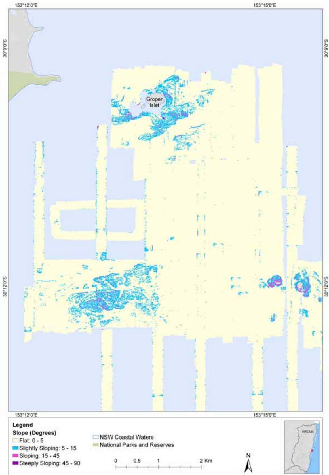
Figure 27. Slope model of the seabed adjacent to and south of South West Solitary (Groper) Island, including Sidney Shoals.
