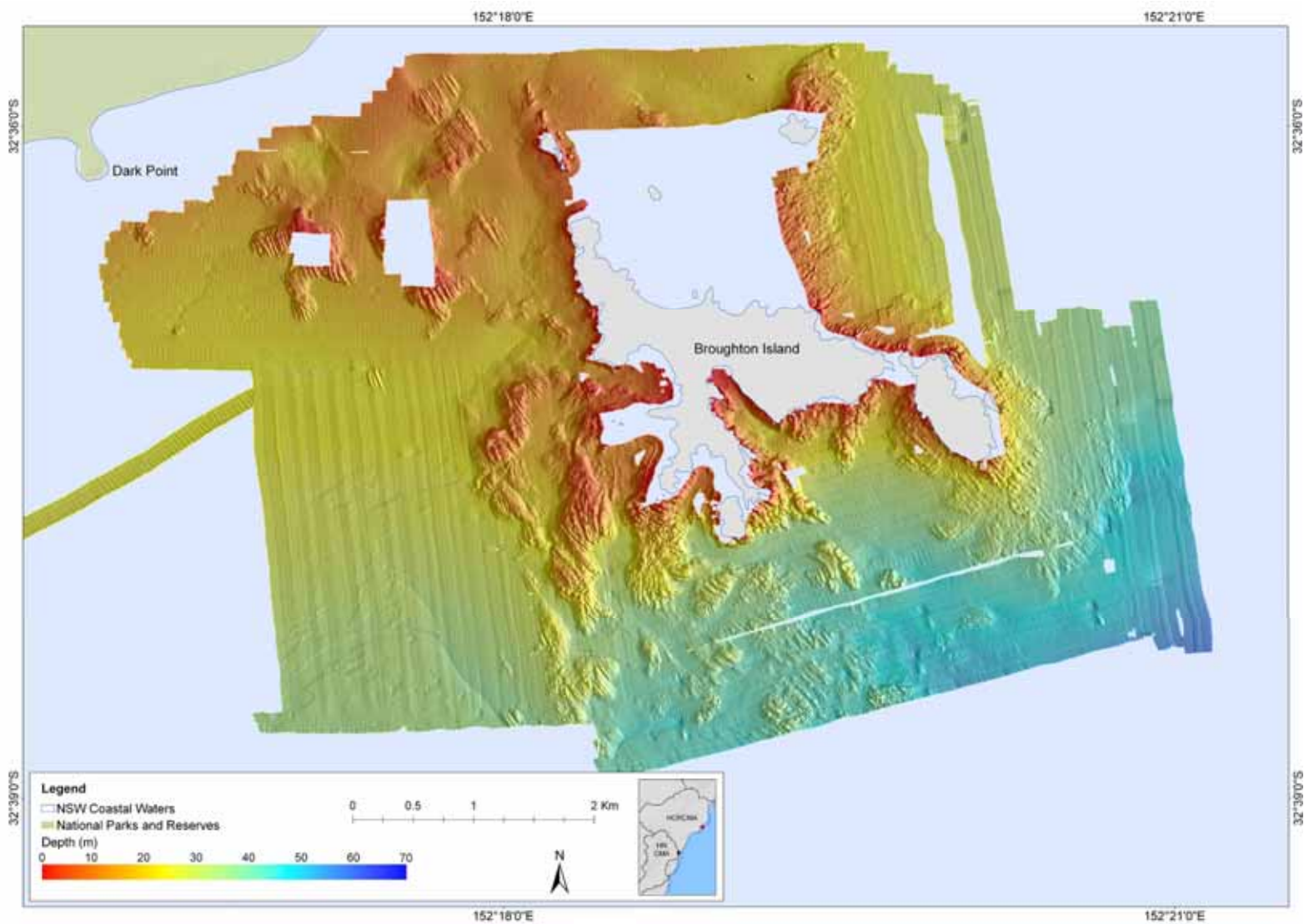
Figure 101. Hill-shaded bathymetric model of the seabed adjacent to Broughton Island.
