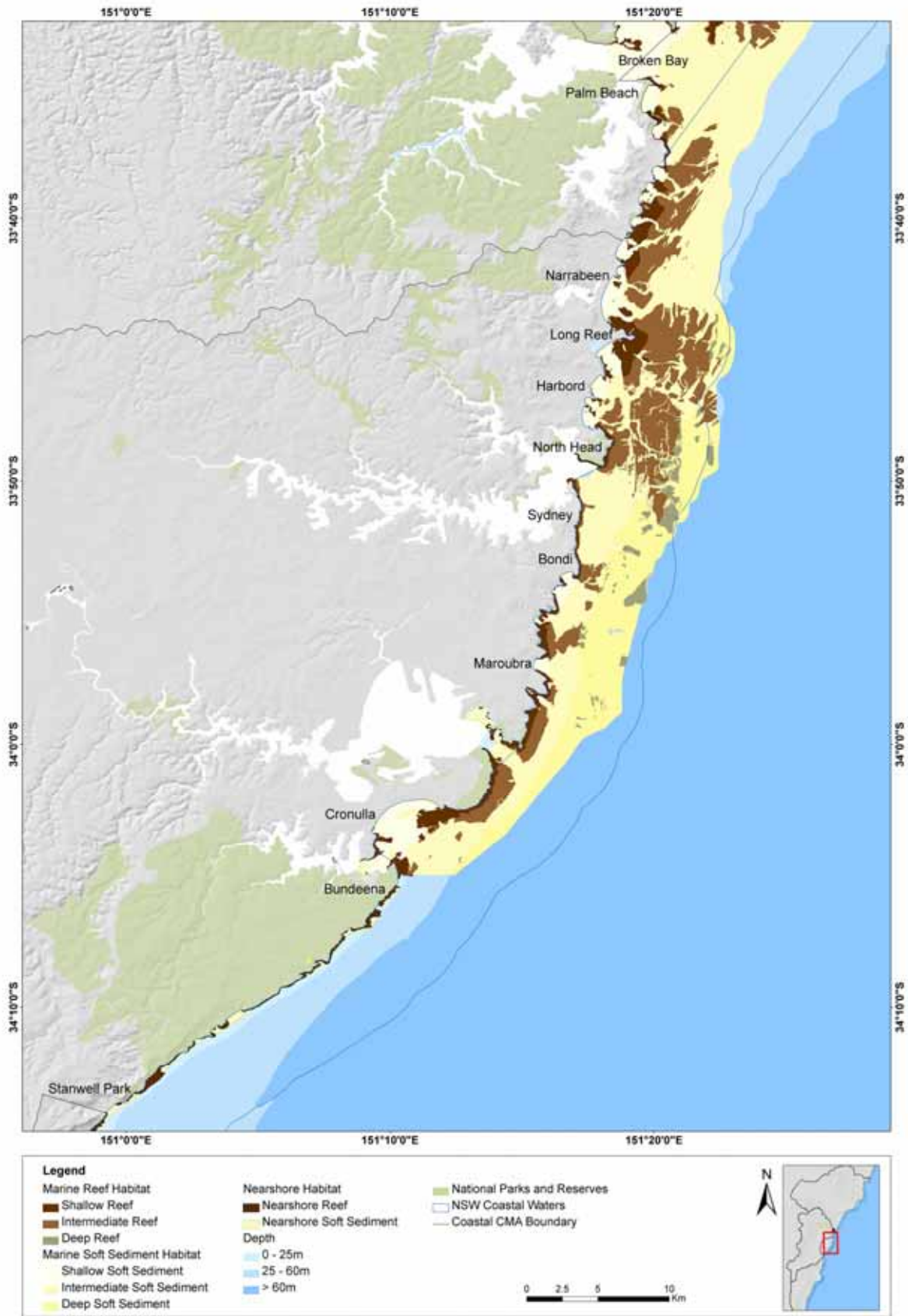
Figure 116. Distribution of known seabed habitats between Broken Bay to Stanwell Park.
