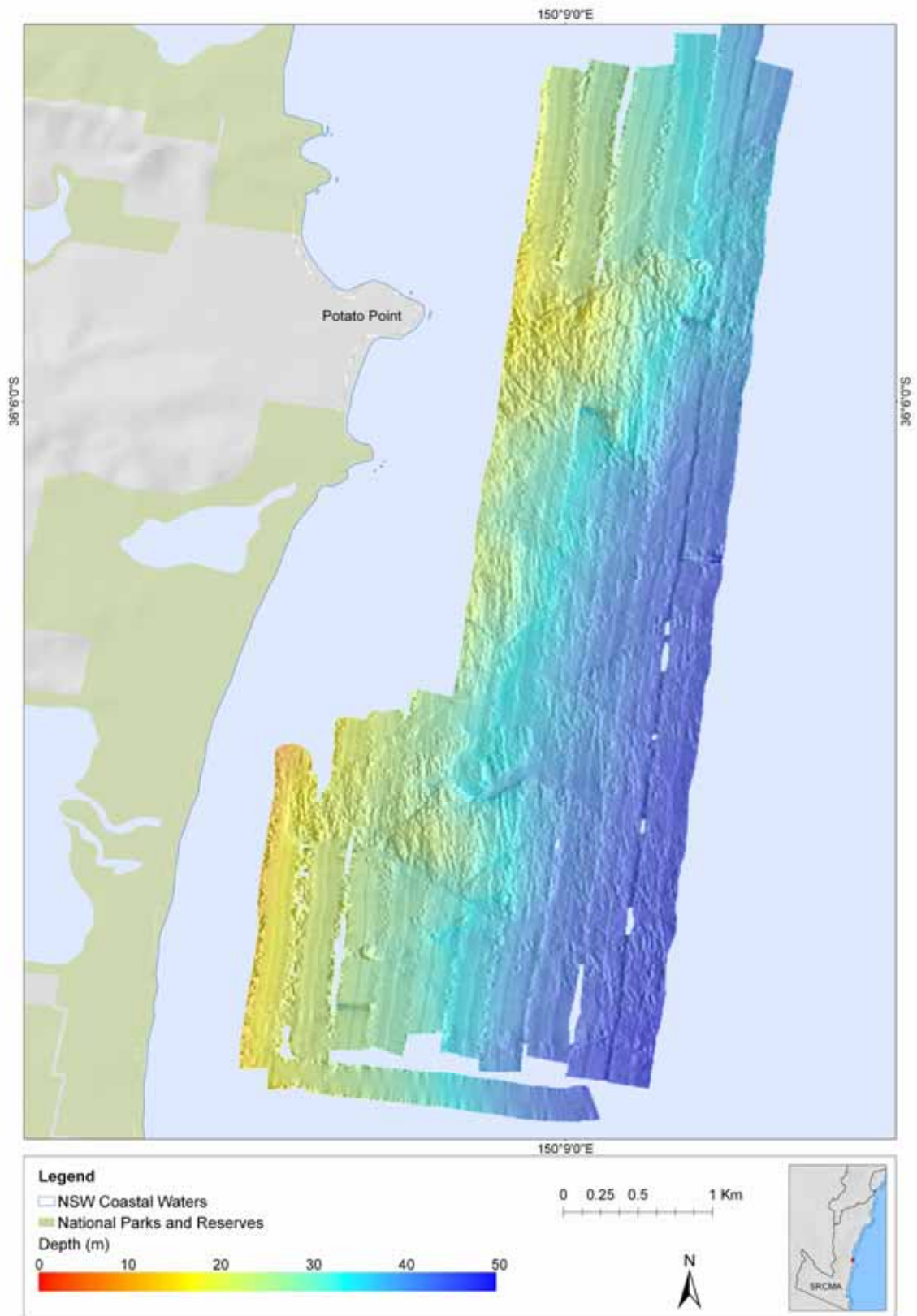
Figure 136. Hill-shaded bathymetric model of the seabed offshore of the Potato Point region.
