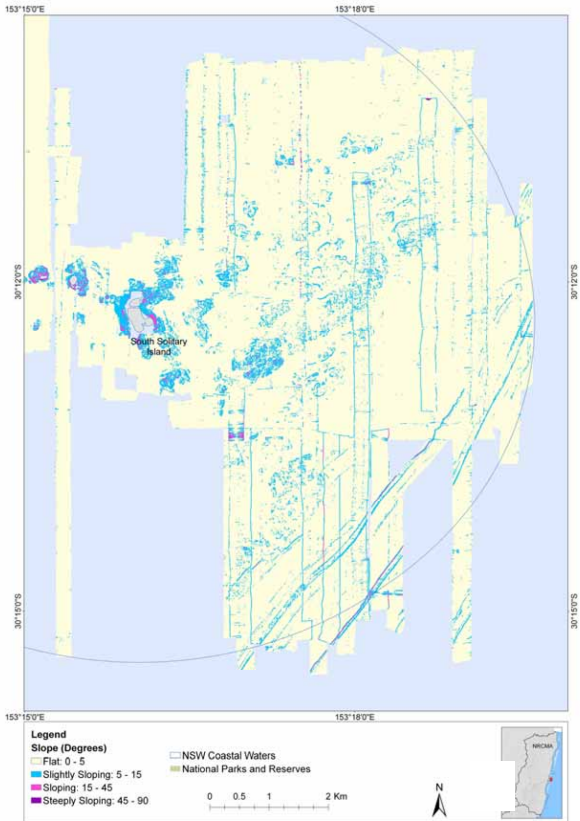
Figure 31. Slope model of the seabed adjacent to and east of South Solitary Island.
