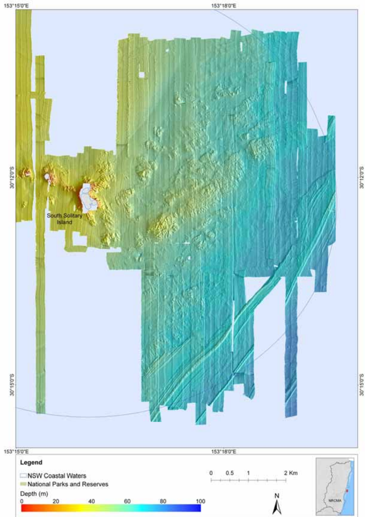
Figure 30. Hill-shaded bathymetric model of the seabed adjacent to and east of South Solitary Island.
