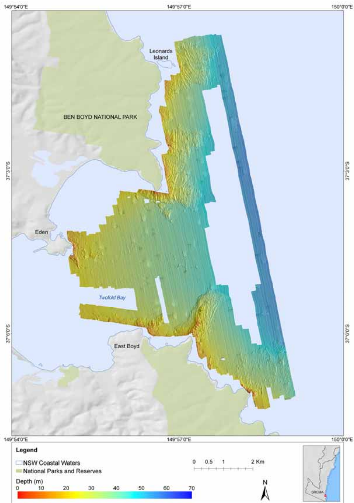
Figure 149. Hill-shaded bathymetric model of the seabed within the Twofold Bay region.
