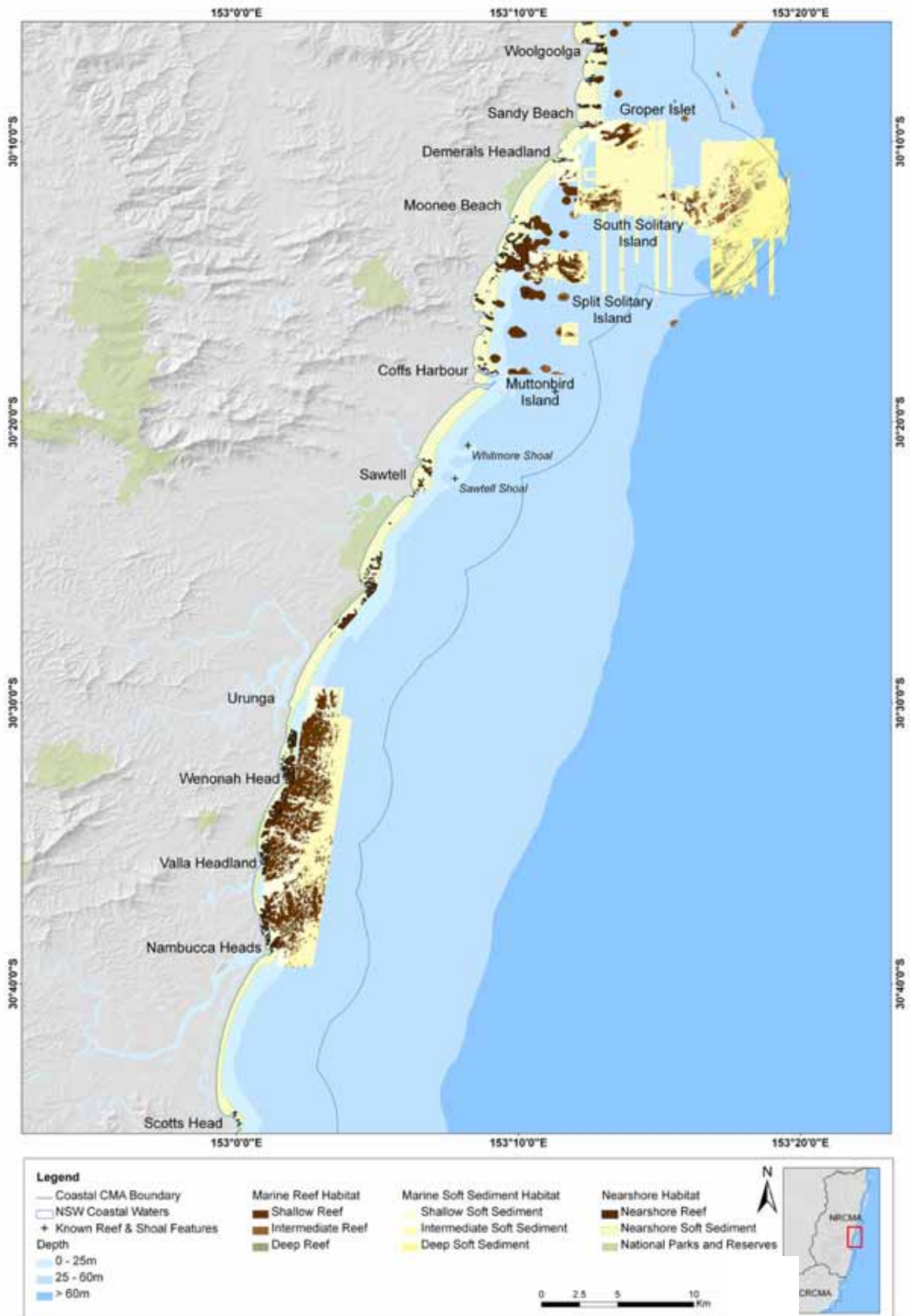
Figure 25. Distribution of known seabed habitats in the region between Woolgoolga and Scotts Head.
