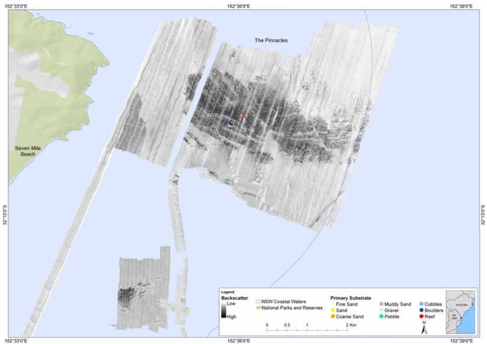
Figure 91. Acoustic backscatter of the seabed surrounding The Pinnacles region.
