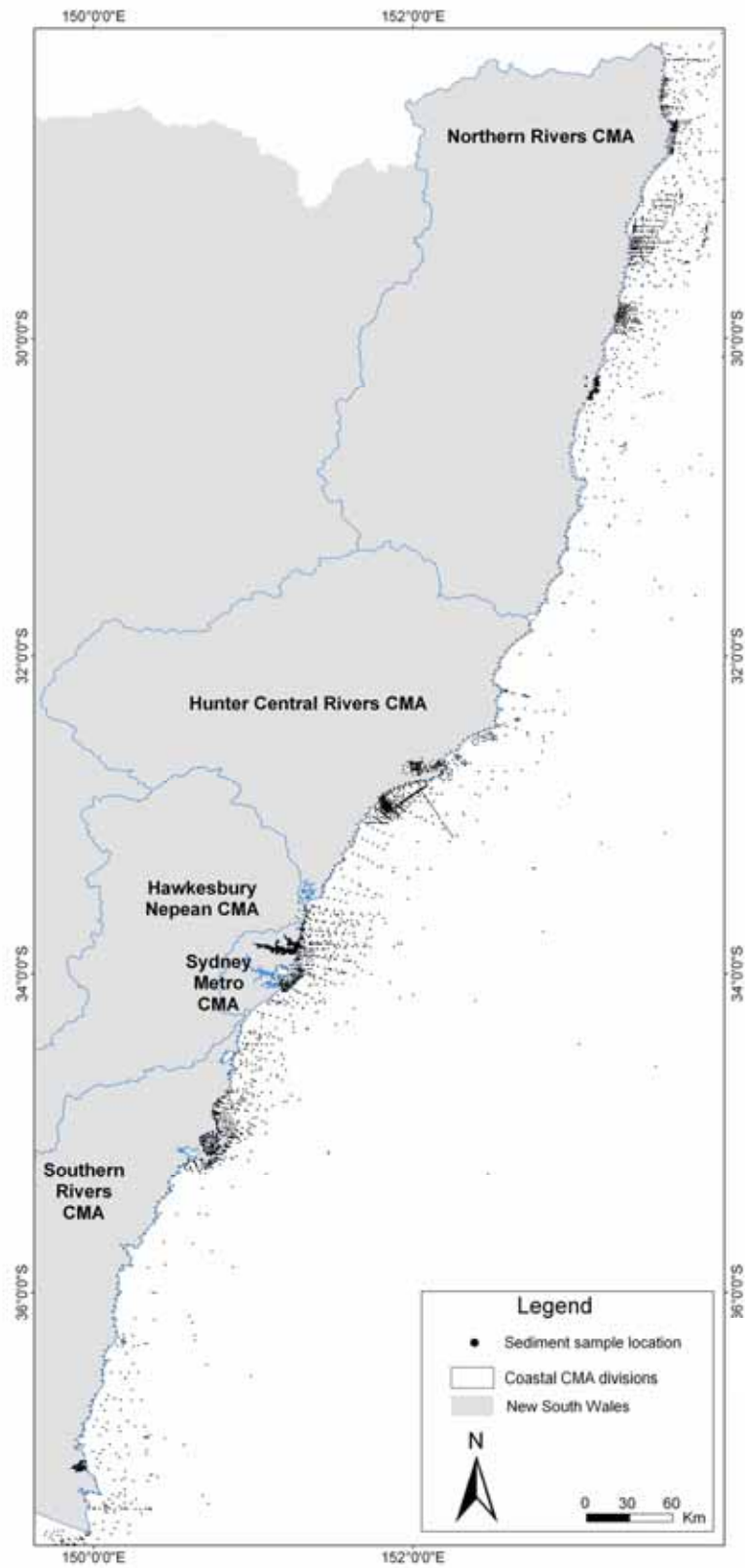
Figure 2. Sediment sample sites used to examine the broadscale distribution of sediments on the NSW continental shelf.
