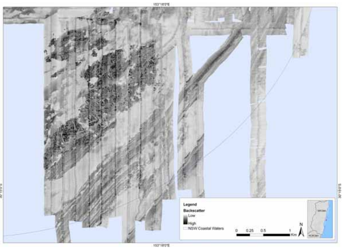
Figure 33. Acoustic backscatter of the seabed adjacent to and east of South Solitary Island.
