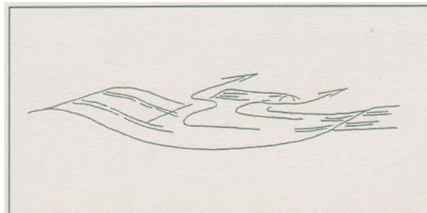
Figure 4: The bank of earth resulting from the spillway clearing can be left to act as a silt trap and water spreader.
