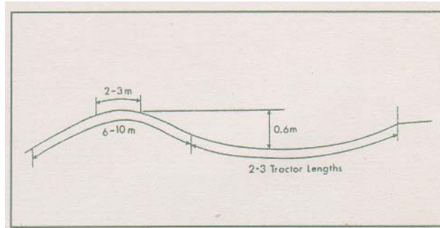
Figure 2: Dimensions of cross banks.
