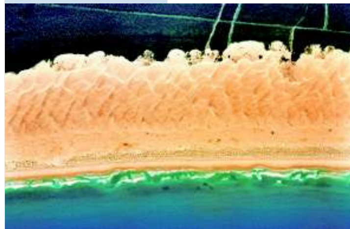
Fig. 2.8b Northward moving sand sheet with eastward moving surface dunes, Stockton Bight.
