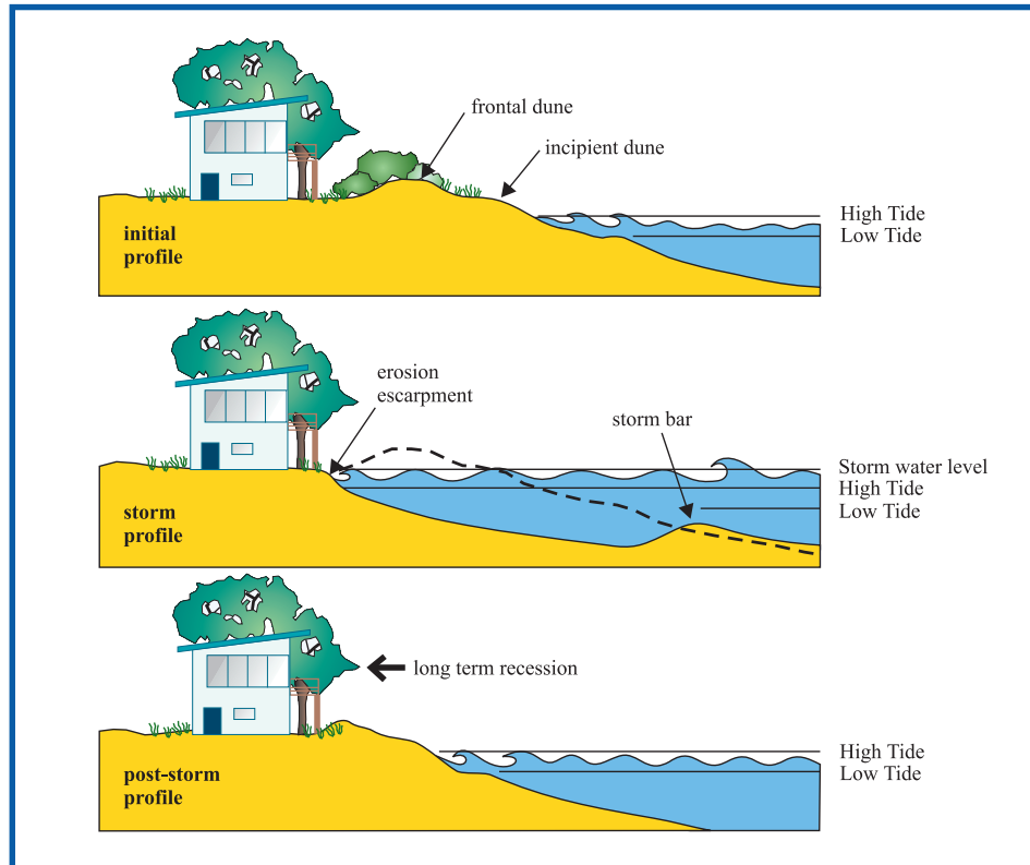
Figure 2.4 Long term beach recession - profile displaced landward due to permanent sand loss.
