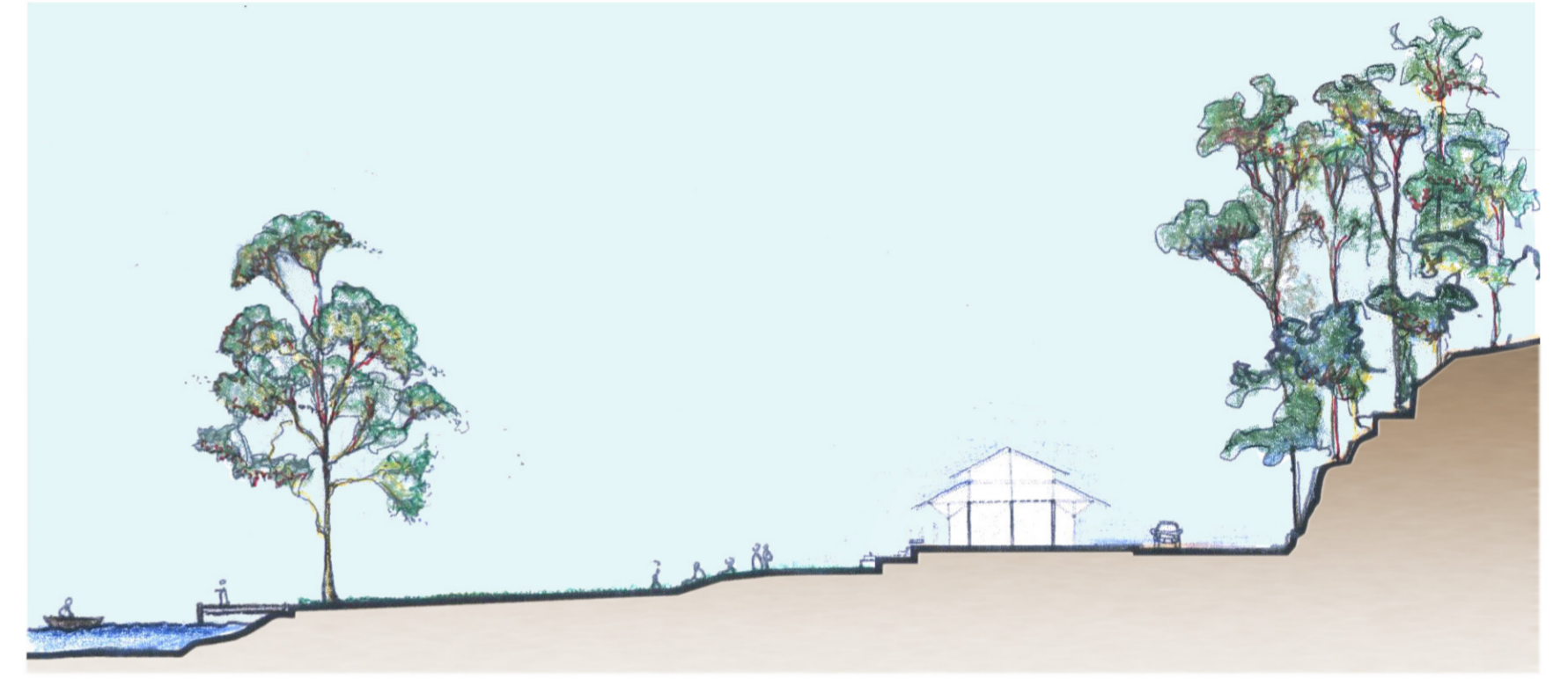
B Section through proposed amenities facility on Pavilion Flat
